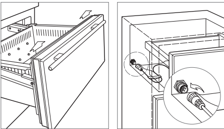
Drawer removal. Control cable (drawers).
