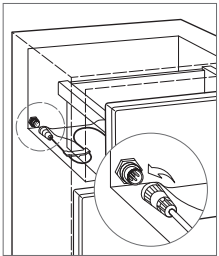
Cable de control (modelo ICB427RG).
